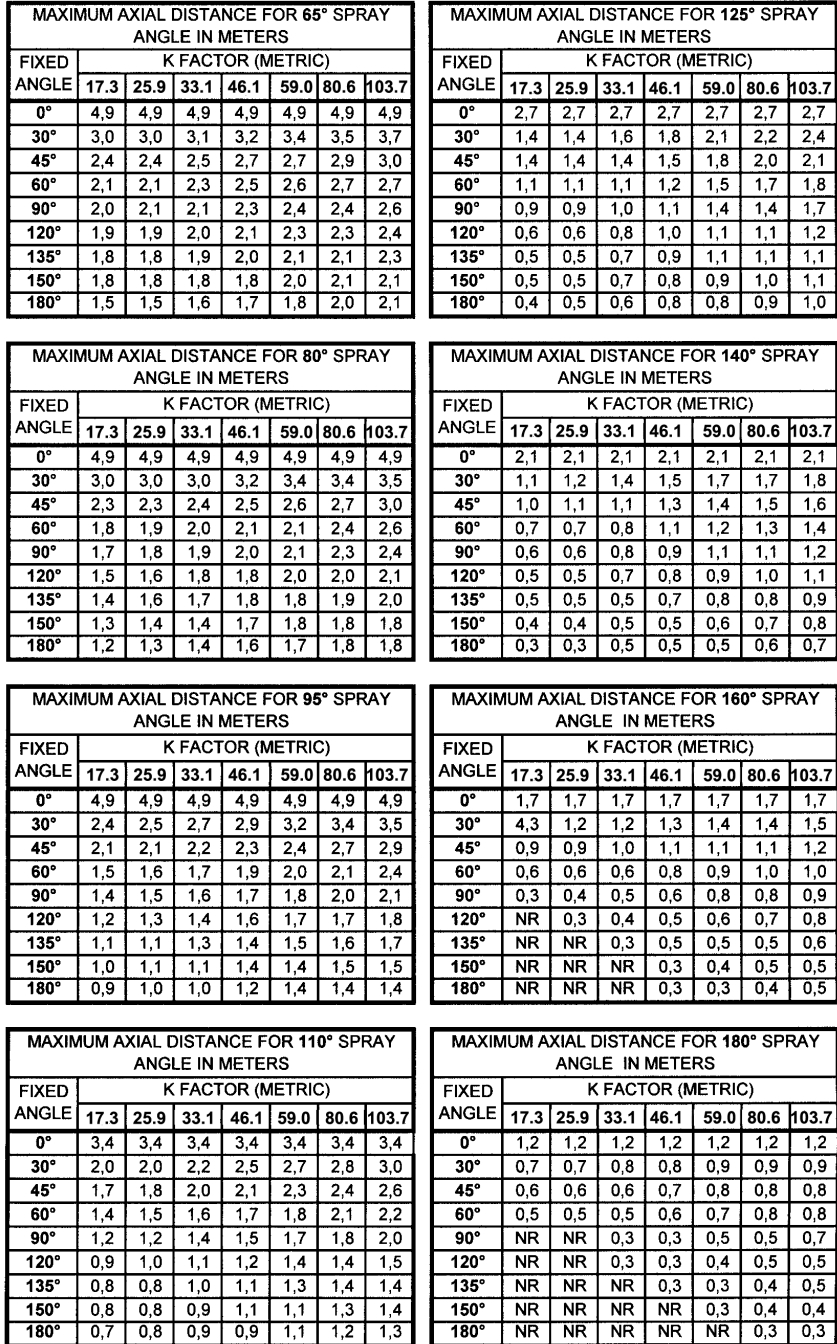
Figure 6b: Maximum Axial Distance Between Nozzle Tip and Plane of Protection for Exposure Protection (m)
